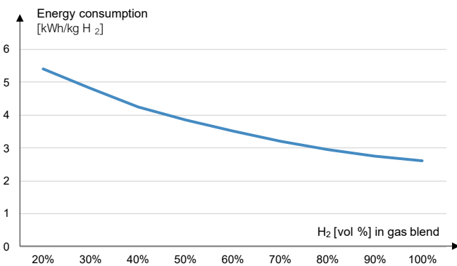
Energy consumption based on hydrogen content [vol %]
