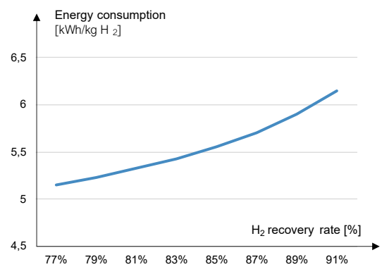
Energy consumption based on recovery rate [%]
